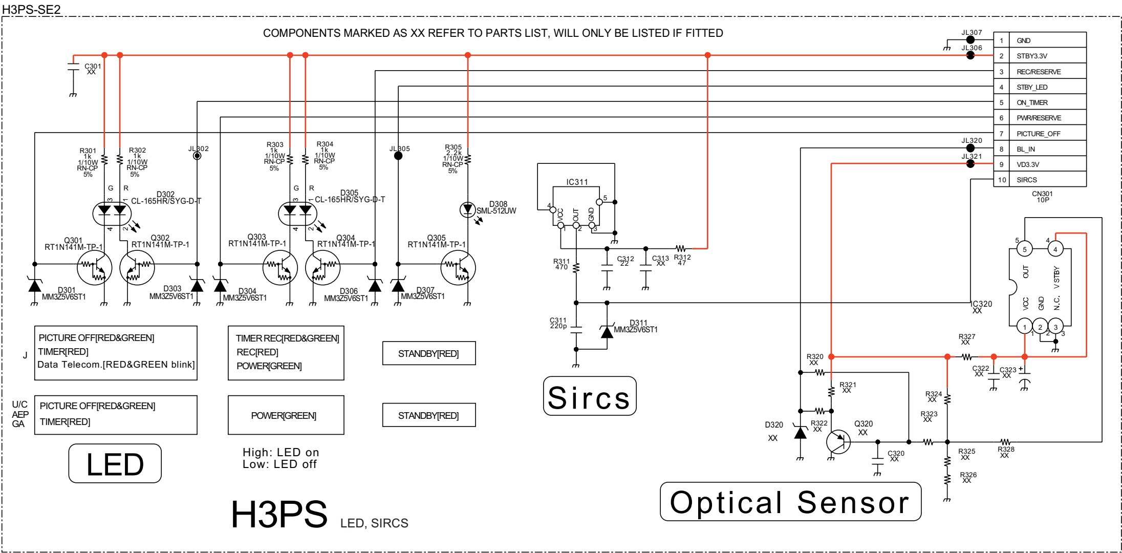
~ H3PS Board Schematic Diagram [ LED, Sircs ] ~
