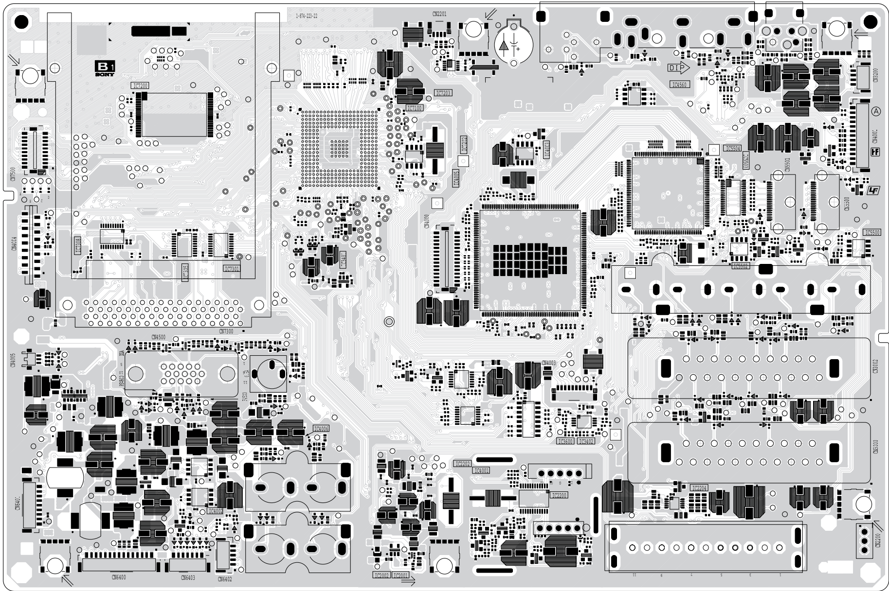
~ B1 Printed Wiring Board Side A ~
