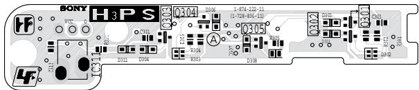
~ H3PS Printed Wiring Board Side A ~
