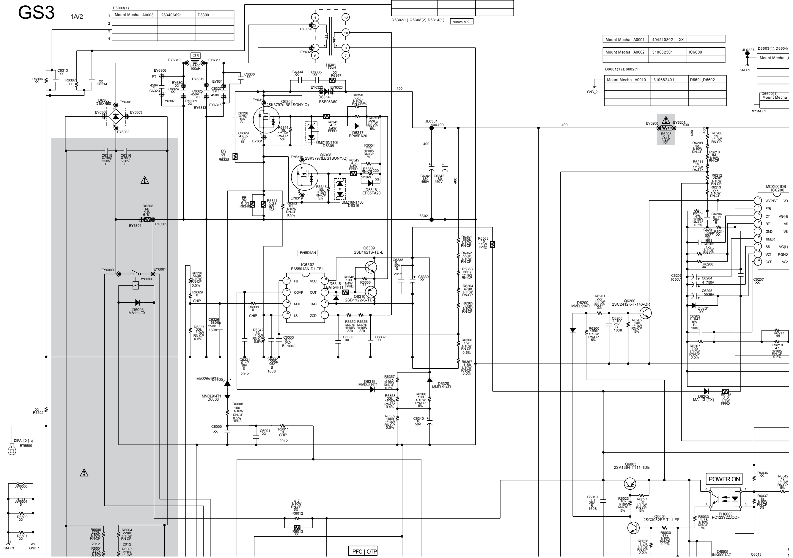
~ GS3 Board Schematic Diagram [ Power Supply ] Page 1A/2 ~
