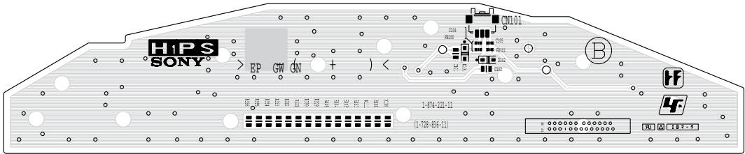
~ H1PS Printed Wiring Board Side B ~
